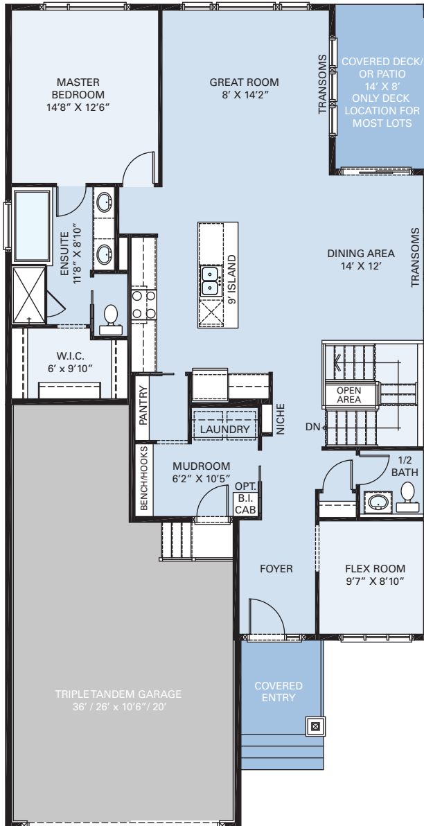
9' MAIN LEVEL
