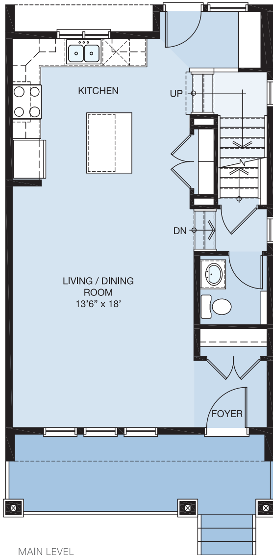
MAIN LEVEL
